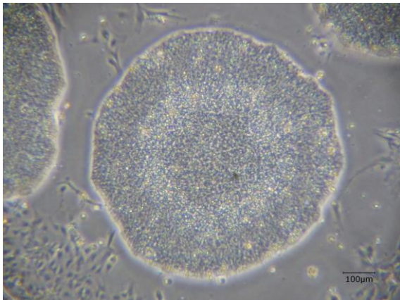
CiRA-j-1240-C: passage-3
